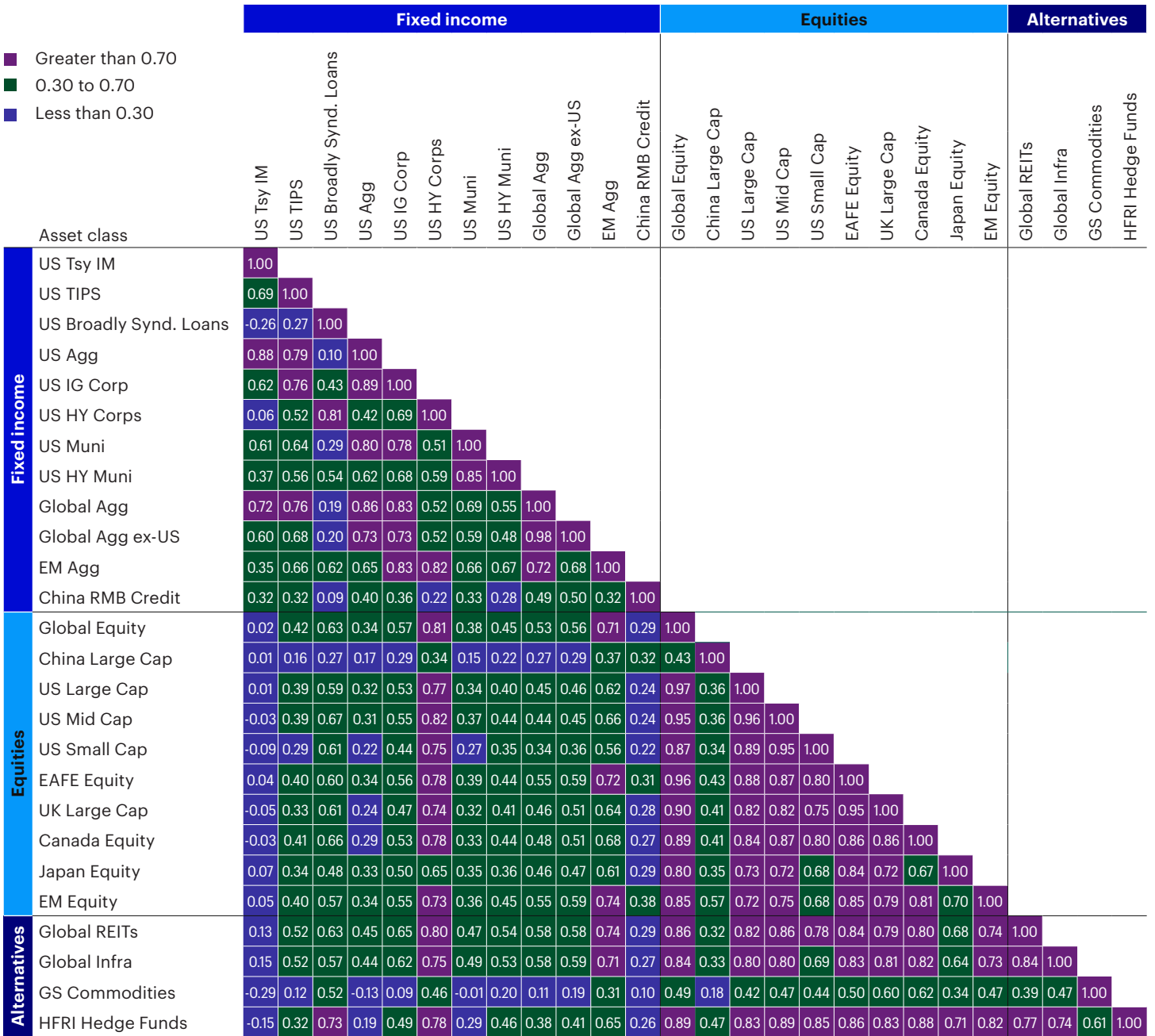
Figure 9: 10-year correlations (GBP)
