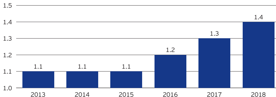
Coverage Ratio 3
